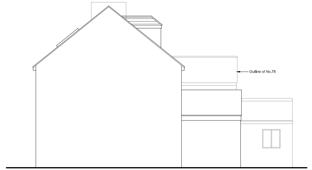
SECTION A-A PROPOSED NORTH ELEVATION 1:100
